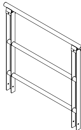
LANDING HANDRAIL
