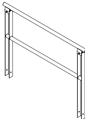
RAMP HANDRAIL 2', 3', 4', & 5'
